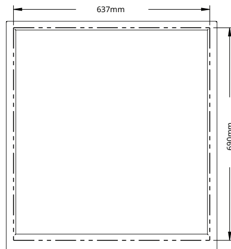
CUT-OUT DIMENSIONS
