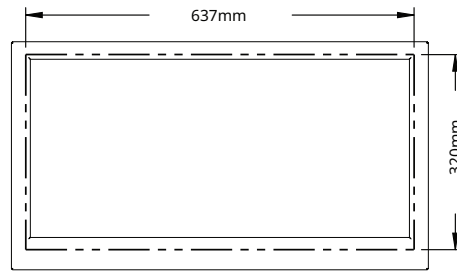
CUT-OUT DIMENSIONS
